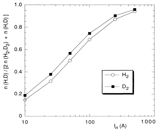
FIG. 5. Fraction of dissociated gas, predicted by the numerical model, as a function of the discharge current I_d .
