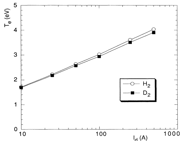
FIG. 1. Temperature of the thermal bulk of the EEDF as a function of the discharge current I_d , from the numerical model.
