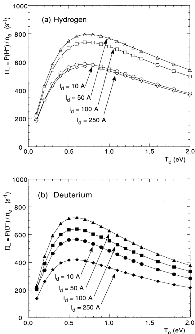
FIG. 7. Production ratio \Pi_- of negative ions [see text and Eq. (2)] from the calculated vibrational spectra and an arbitrary Maxwellian EEDF as a function of T_e , for (a) hydrogen discharge and (b) deuterium discharge.
