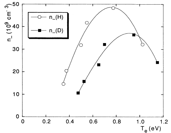
FIG. 14. Negative-ion density n_- plotted against electron temperature T_e , both measured in the extraction region of a tandem source.
