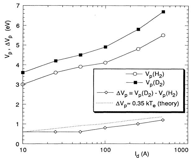
FIG. 4. Plasma potential in hydrogen and deuterium discharges as a function of the discharge current I_d , from the numerical model. Following the analysis of Ref. [13], \Delta V_p is also plotted and compared with simple theory [33] for no magnetic confinement.
