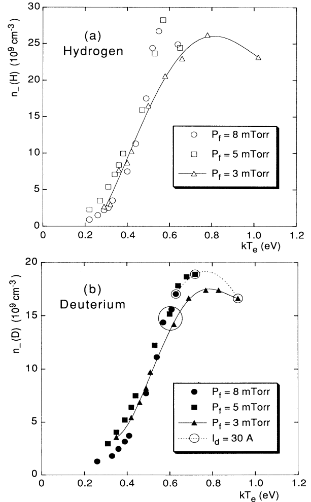
FIG. 13. Measured negative-ion density n_- , for several values of filling pressure P_f , as a function of the measured electron temperature T_e . All measurements made at the center of the hybrid source in (a) a hydrogen discharge and (b) a deuterium discharge. The four data points enclosed by the large circle in (b) are discussed in the text.
