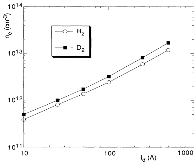
FIG. 2. Plasma density as a function of the discharge current I_d from the numerical model.
