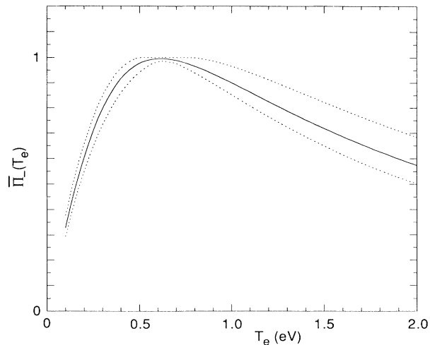
FIG. 8. —, plots average of \bar{\Pi}_- over the ensemble of calculations (hydrogen and deuterium discharges with I_d = 10, 50, 100, and 250 A and P_f = 3 mTorr), while \cdot \cdot \cdot indicates the maximum and minimum values of \bar{\Pi}_- over the same ensemble.
