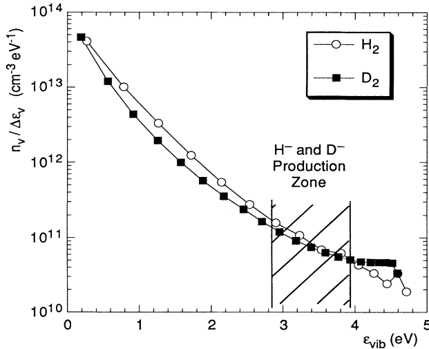
FIG. 6. Vibrational spectra, with vibrational populations normalized to spacing between vibrational levels (see text), predicted by the model for the P_f = 3 mTorr, I_d = 50 A case. Hatched area indicates vibrational levels principally responsible for negative-ion creation via DA.
