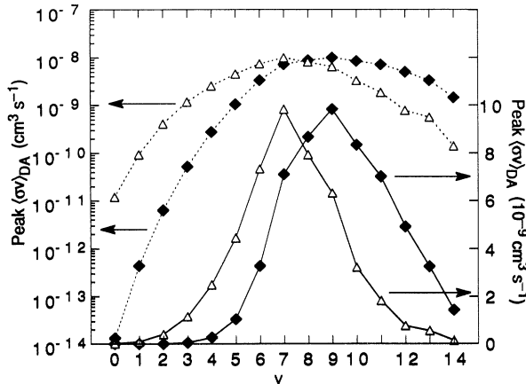
FIG. 10. At each vibrational level v'' of hydrogen, \blacklozenge indicates the maximum value attained by \langle \sigma v \rangle_{\text{DA}} as T_e is varied, on both logarithmic ( \cdots \blacklozenge \cdots ) and linear ( \text{---} \blacklozenge \text{---} ) scales. The effect of weighting these peak values by the vibrational populations of a “typical” spectrum H_2(v'') (that of Fig. 6, see text) is indicated by \triangle . The weighted values are arbitrarily renormalized for convenient display and plotted on both logarithmic ( \cdots \triangle \cdots ) and linear ( \text{---} \triangle \text{---} ) scales.
