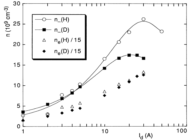
FIG. 12. Negative-ion density n_- and scaled-down electron density n_e measured in the hybrid source as a function of the discharge current I_d , at P_f = 3 mTorr.
