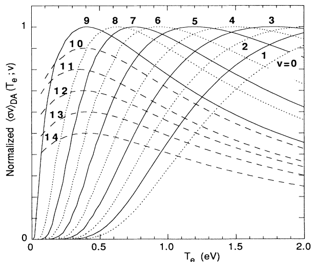
FIG. 9. — and \cdot \cdot \cdot show the T_e dependence of the dissociative attachment rate coefficients \langle \sigma v \rangle_{\text{DA}} for hydrogen used in the numerical model, normalized to unity for v'' \leq 9 . The v'' \geq 10 rate coefficients for exothermic attachment, indicated by - - - , have a similar T_e dependence and are normalized to 0.9, 0.8, \dots, 0.5 to distinguish them on the plot.
