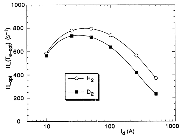
FIG. 11. The optimum production ratio \Pi_-(T_e = T_e^{\text{opt}}) predicted by the numerical model for hydrogen and deuterium.
